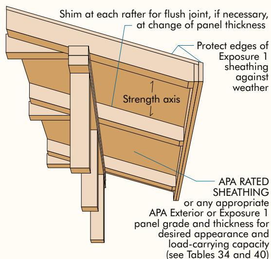
FIGURE 26 OPEN SOFFIT
