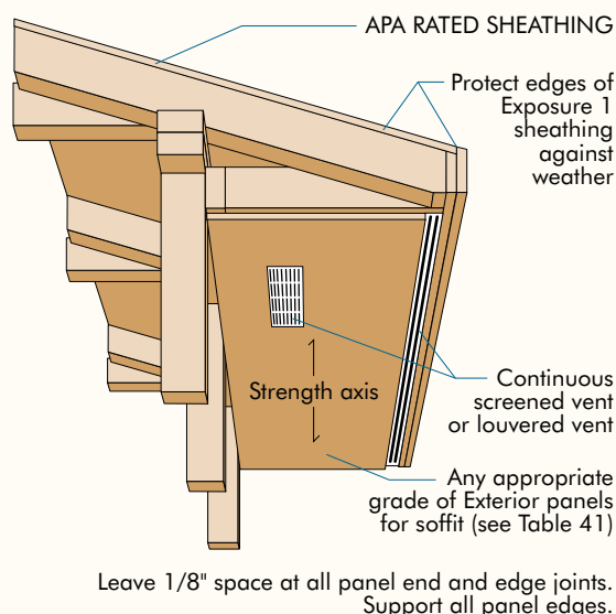
FIGURE 27 CLOSED SOFFIT
